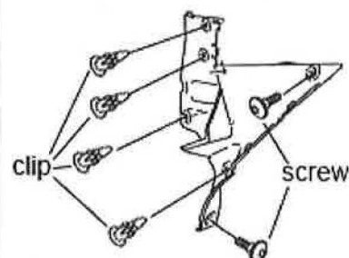
inner fairing (cowl)
